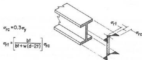
Figure 12: Ketter Residual Stress Pattern
